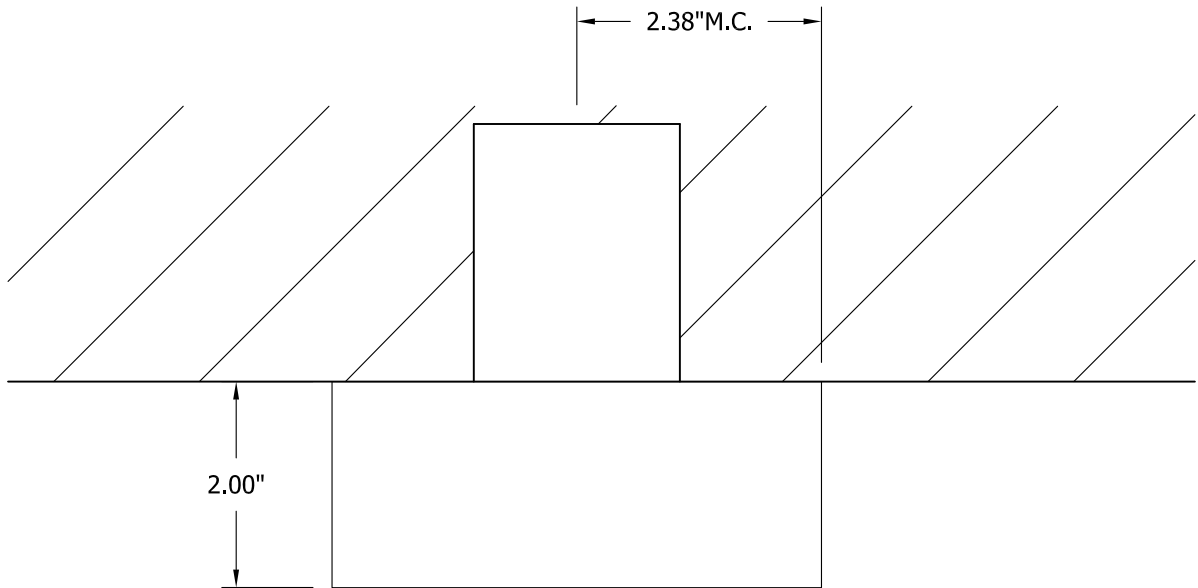
FRONT VIEW
