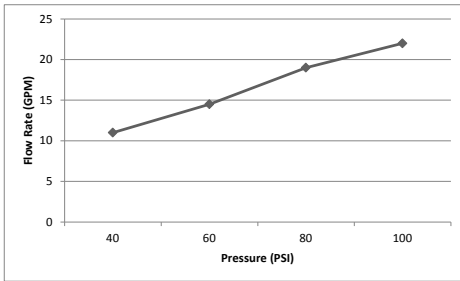
P-1131B Flow Rate (GPM) Vs Pressure (PSI)*
