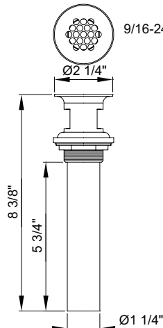
Grid Strainer
