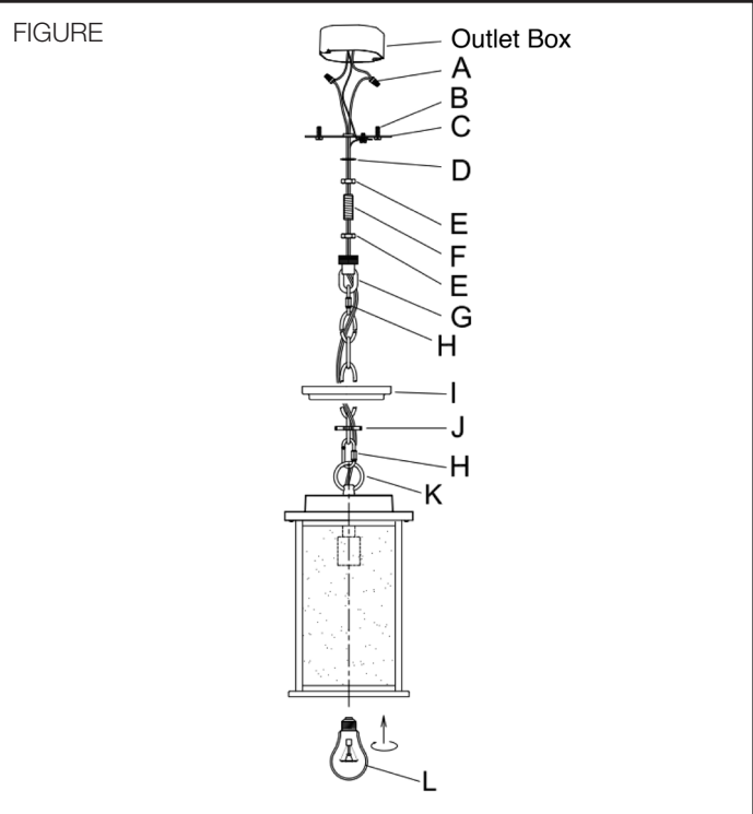
FIGURE Line art shown may not exactly match the fixture enclosed. However, the installations do apply to this fixture.
