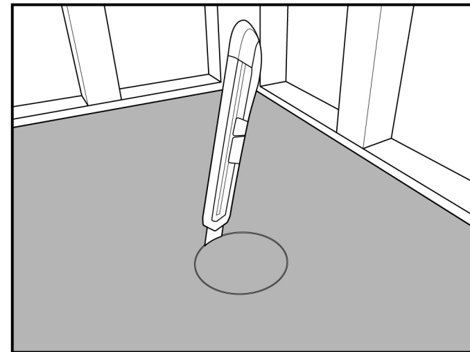
STEP 03: Cut out the drain hole and tack around the edges.
