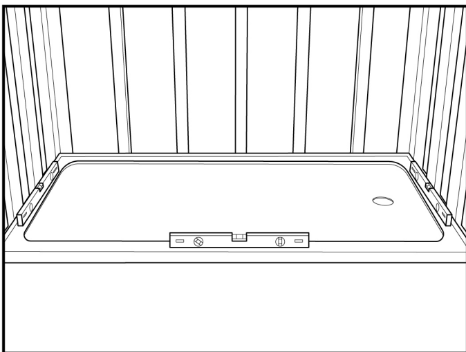
STEP 04: Dry fit the shower base and check to see if the subfloor is level.
