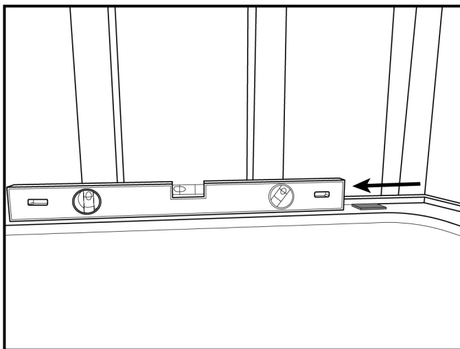
STEP 05: Use the level to determine the thickness of the shims required to level the shower base
