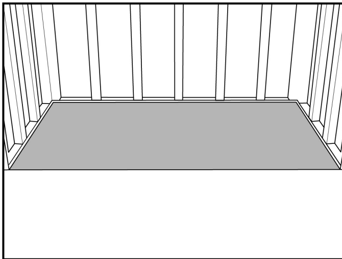
STEP 02: Cut tar paper to size and tack onto the sub floor.
