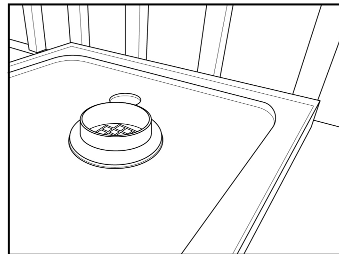
STEP 06: Apply silicone caulking to the underside of the drain flange. Note drain not included with base.
