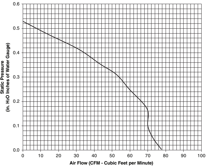
Model AN70L
