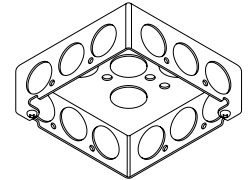
4" Square
