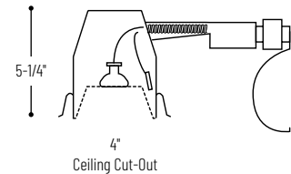
Ceiling Cut-Out
