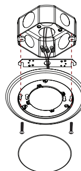
Figure 3 Mount luminaire to junction box with screws.
