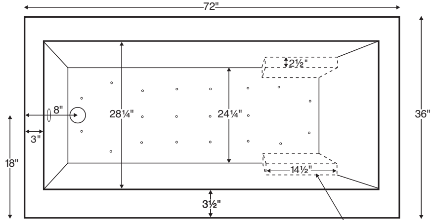
Optional Integral Armrests
