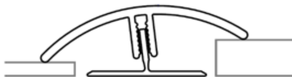
REDUCER
