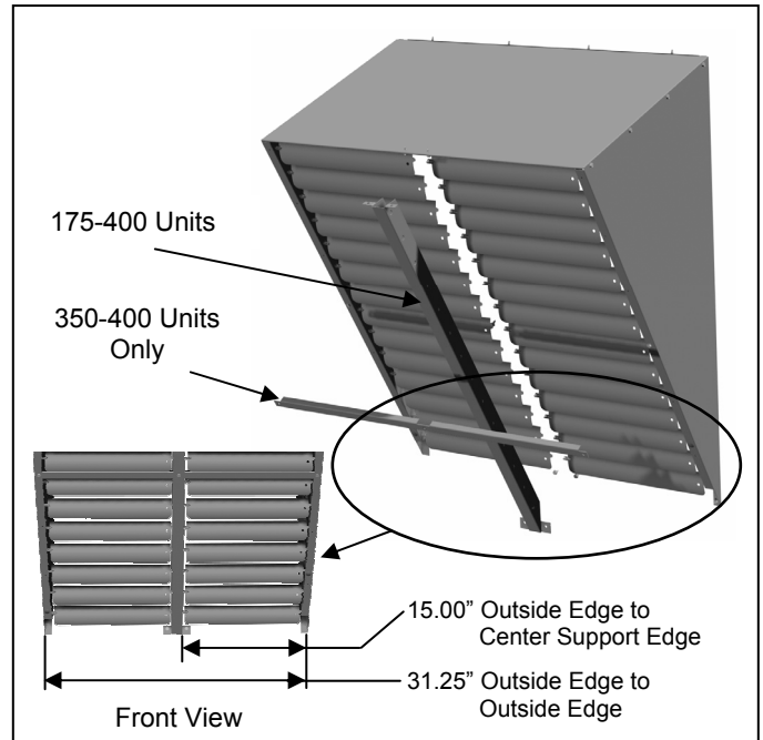
Figure 2.3 – Deflector Bracket and Cross Member
