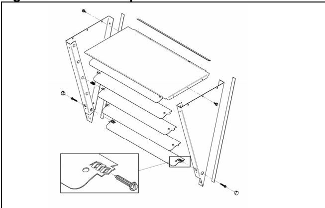
Figure 2.2 - Hood to Unit Exploded View
