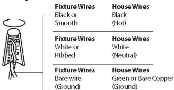
Fig.2 Wiring
