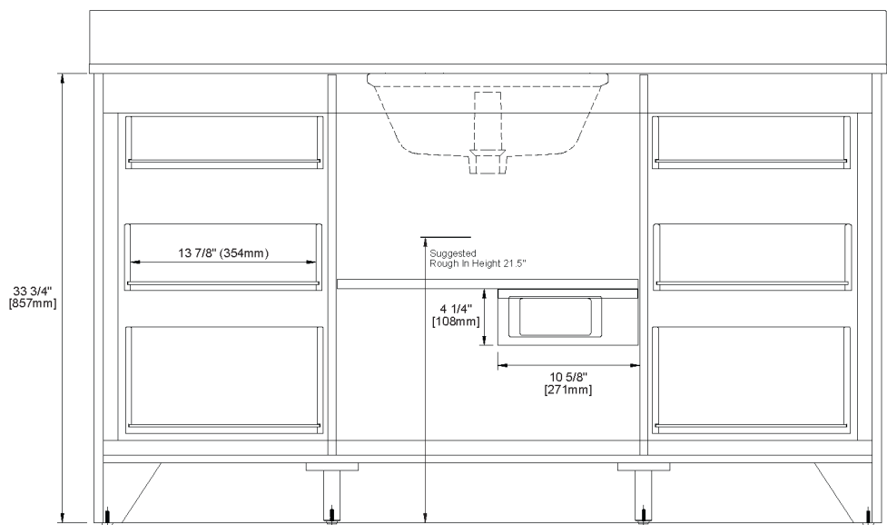
Back View
