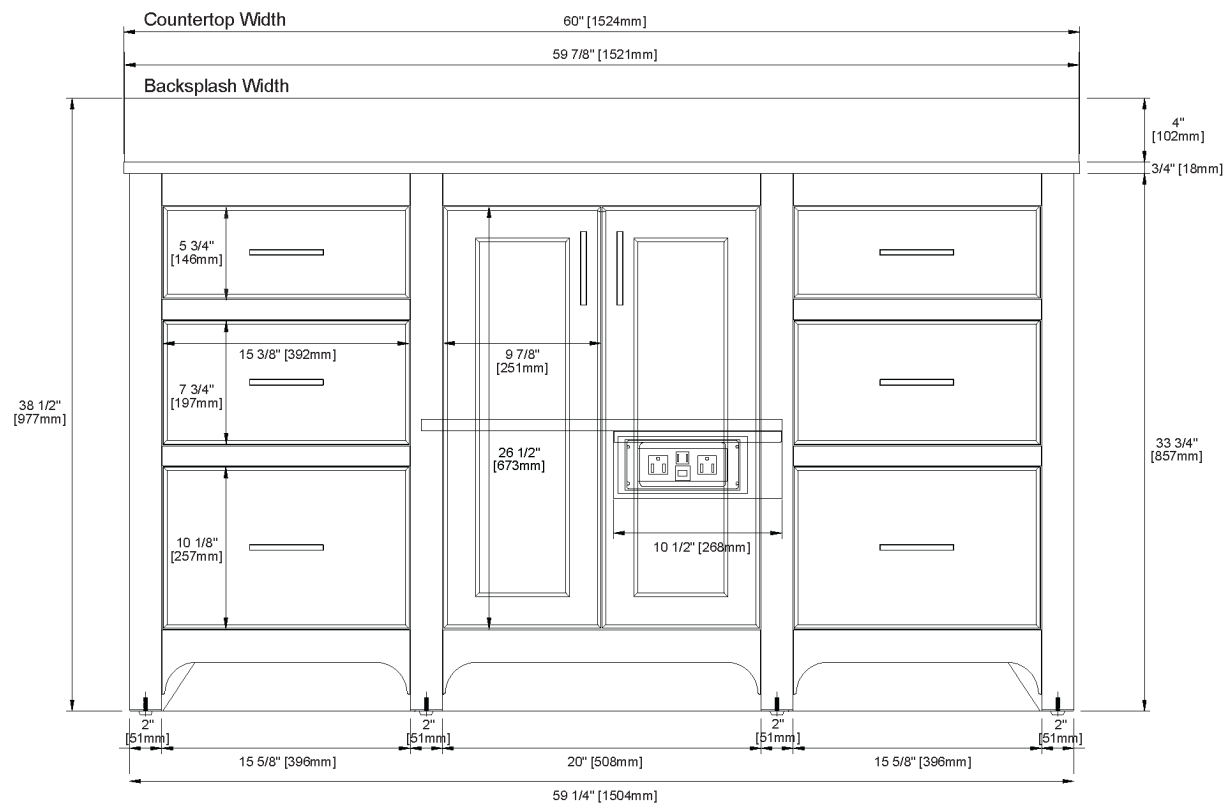
Front View
