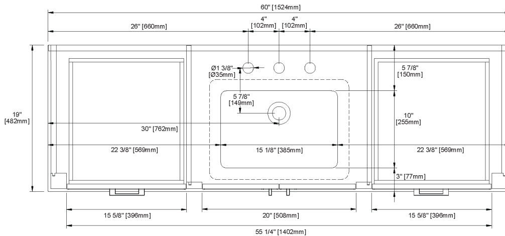
Top View
