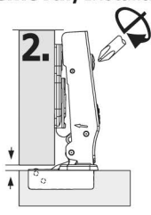
2. Adjustable cassette/ Cassette réglable +0.11 -0.04 Cassette/Cassette +0.11 -0.08
