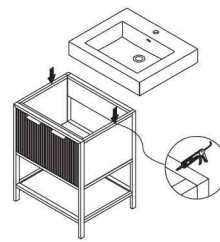
1. Paste the countertop Coller le comptoir
