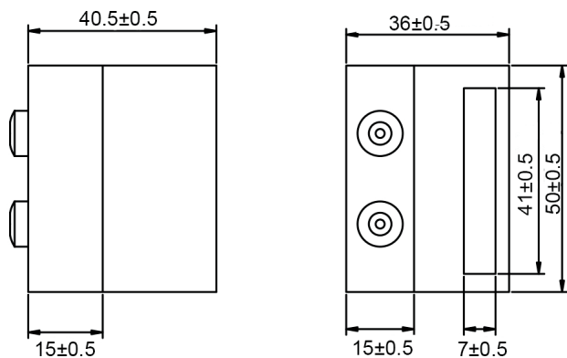
Flat Rail Stop Standard
