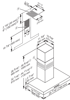
PUR 88 W (Installation drawing) – USA/CDN
