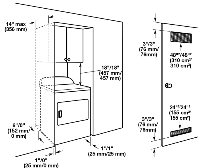
Recommended/Minimum spacing
