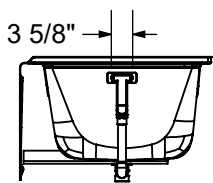
INTEGRATED LINEAR OVERFLOW & DRAIN OPTION
