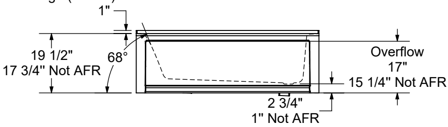
INTEGRATED LINEAR OVERFLOW & DRAIN OPTION
