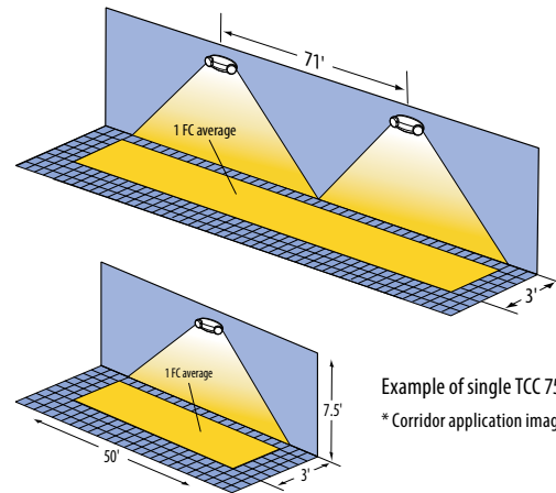
Example of multiple TCC 750L luminaires illuminating a 3' path of egress.
