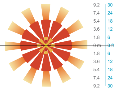
15 FT MOUNTING
