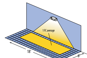
Example of single LHQM LED WRS exit illuminating a 6' path of egress
