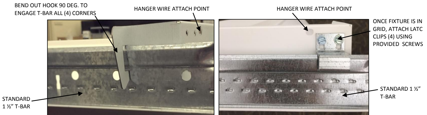
Figure 2: LATC Installation (ORDERABLE OPTION)
