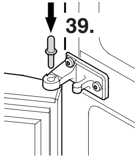
39. Insert middle hinge pin.
