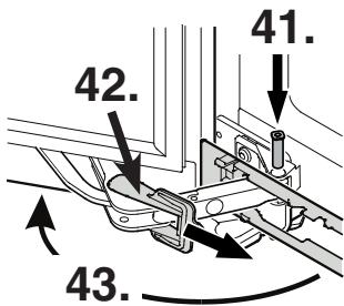
41. Move soft stop mechanism hinge to the fastener and insert pin.
