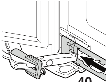
40. Slide door cover over soft stop mechanism hinge.
