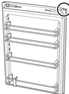
48. Feed in the cable of the hinge at the opposite side and insert hinge.
