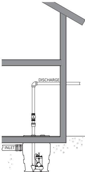
Figure 3. Typical Sump Installation (variations may apply)
