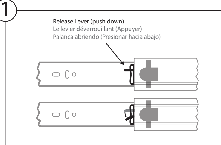
1. Press release lever (shown above) to disconnect drawer members.
