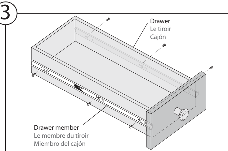
3. On drawer place and align drawer member into position. Place drawer member end flush with the drawer overlay. Fasten each drawer member with (3) #6 pan head wood screws.
