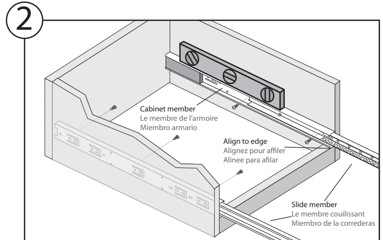
2. Using a level, place and align cabinet member into position and place side flush with the cabinet edge. Fasten each slide with (3) #6 pan head wood screws. You will need to move the slide member back and forth to access the screw holes. For supporting heavy objects use (5) #8-32 machine screws and inserts to avoid tear out of slide.
