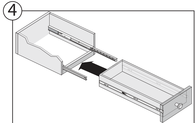
4. Insert drawer into cabinet and close. The drawer slide release lever will lock as drawer is closed. Make sure drawer aligns properly and rides smoothly on the side mount drawer slides.
