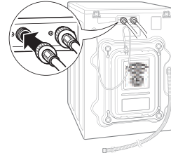
Connecting the water line
