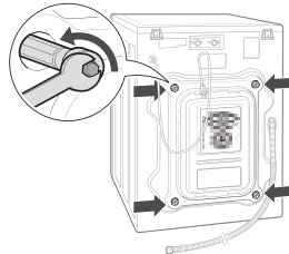
Unpacking and removing shipping bolts
