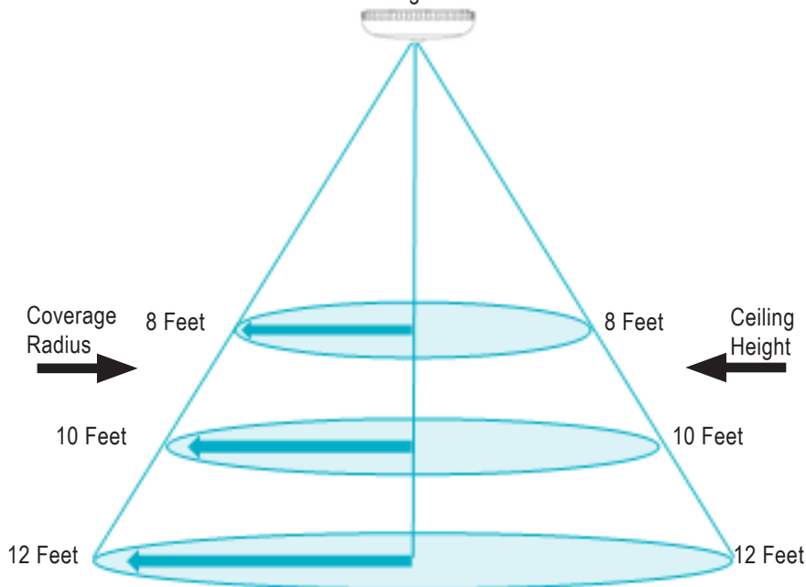
Figure 13: Ceiling Sensor Detection Zones 45 degrees
