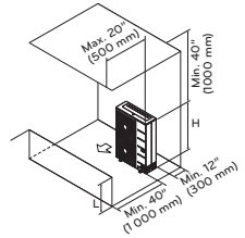
Series installation.
