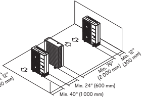
Series installation.
