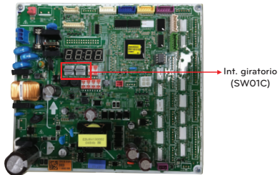
PCB principal (maestro)
