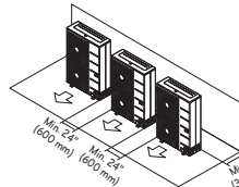
Side-by-side series installation.
