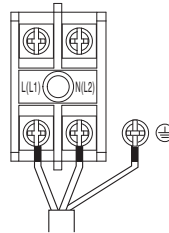
Power Supply High Voltage (208/230)
