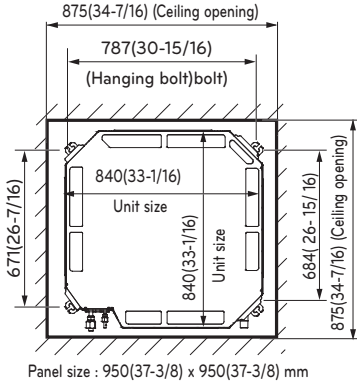
[24-48 kBtu/h] Unit: mm (inch)
