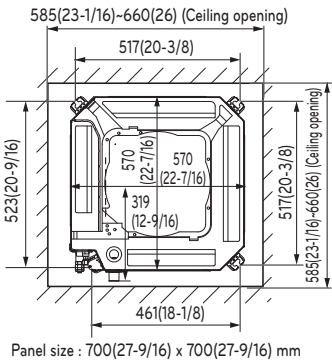
[7-18 kBtu/h] Unit: mm (inch)
