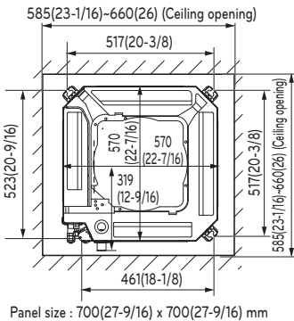
[7-18 kBtu/h] Unit: mm (inch)
