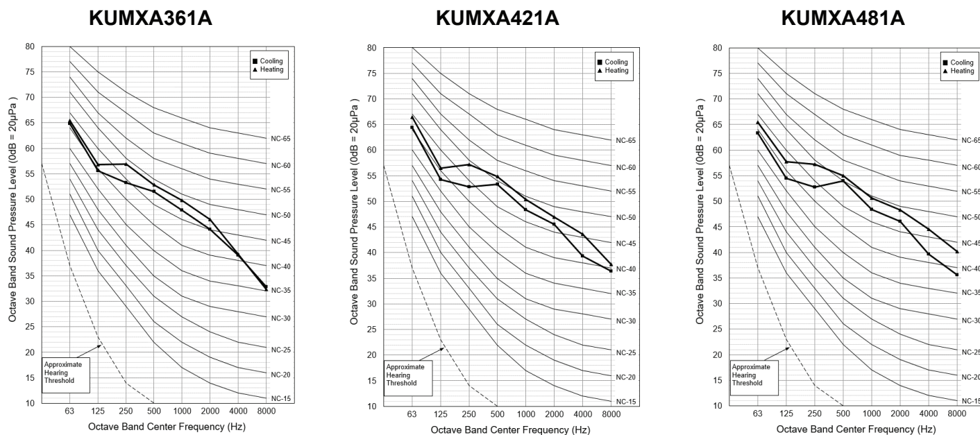
Figure 19: Sound Pressure Level Diagrams.
