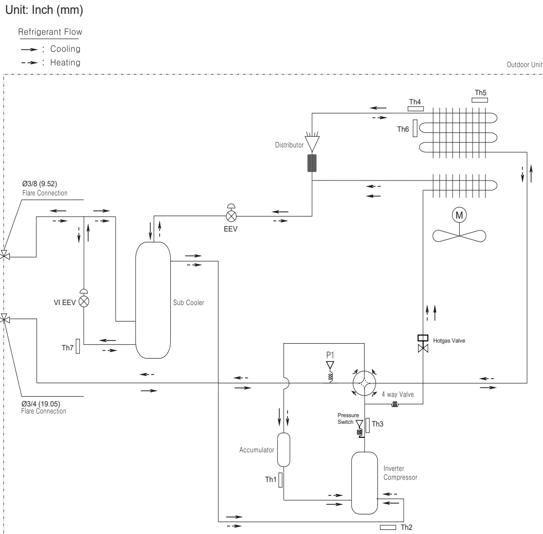
Figure 17: KUMXA361A, KUMXA421A, and KUMXA481A Refrigerant Flow Diagram.
