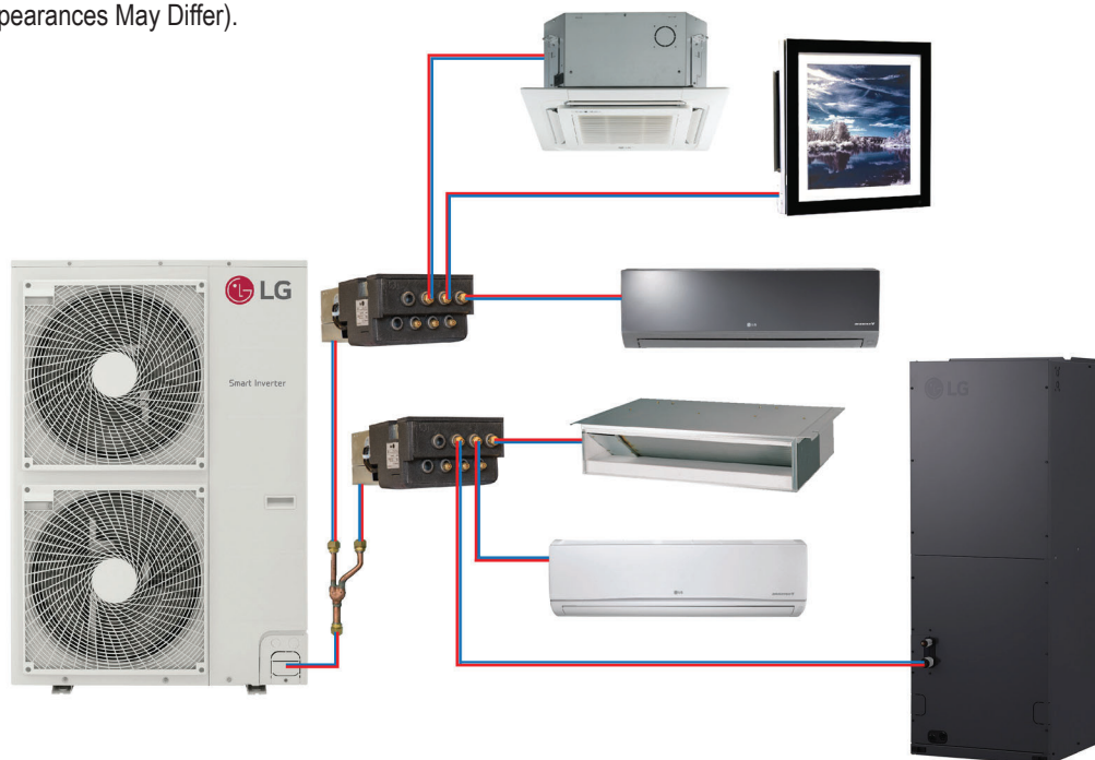
Figure 4: KUMXB481A, (18,000-65,000 Btu/h), KUMXB541A (18,000-73,000), and KUMXB601A (18,000-81,000) Multi F MAX Heat Pump Inverter Outdoor Units (Appearances May Differ).
