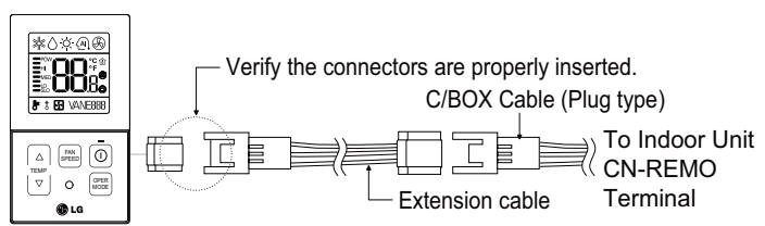
Figure 118: PZCWRC1 LG Wired Remote Extension Cable.
