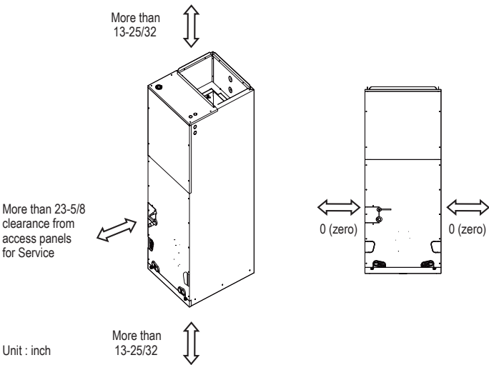
Figure 228:Clearance Requirements.
