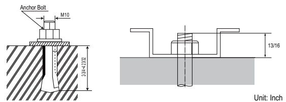
Figure 255: Close up of Bolt Attachment.
