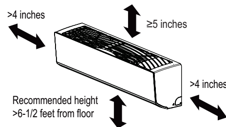
Figure 72: Minimum Clearance Requirements.
