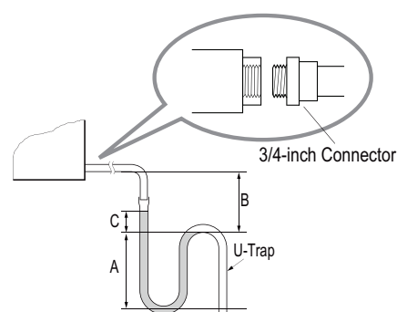
Figure 239: Installing the U-Trap.
