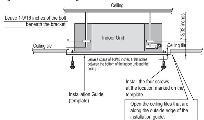
Figure 198: Installation Diagram.
