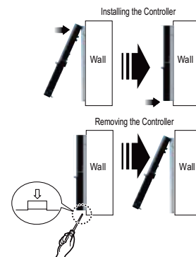
Figure 217: Installing / Removing the Controller.
