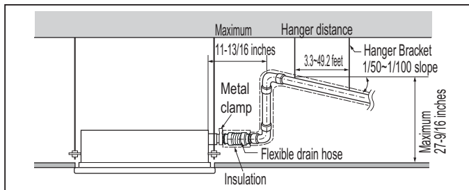
Figure 140: Drain Piping Installation Dimensions.
