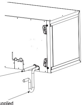
Figure 209: Insulating the Refrigerant Piping and Refrigerant Piping Connections.
