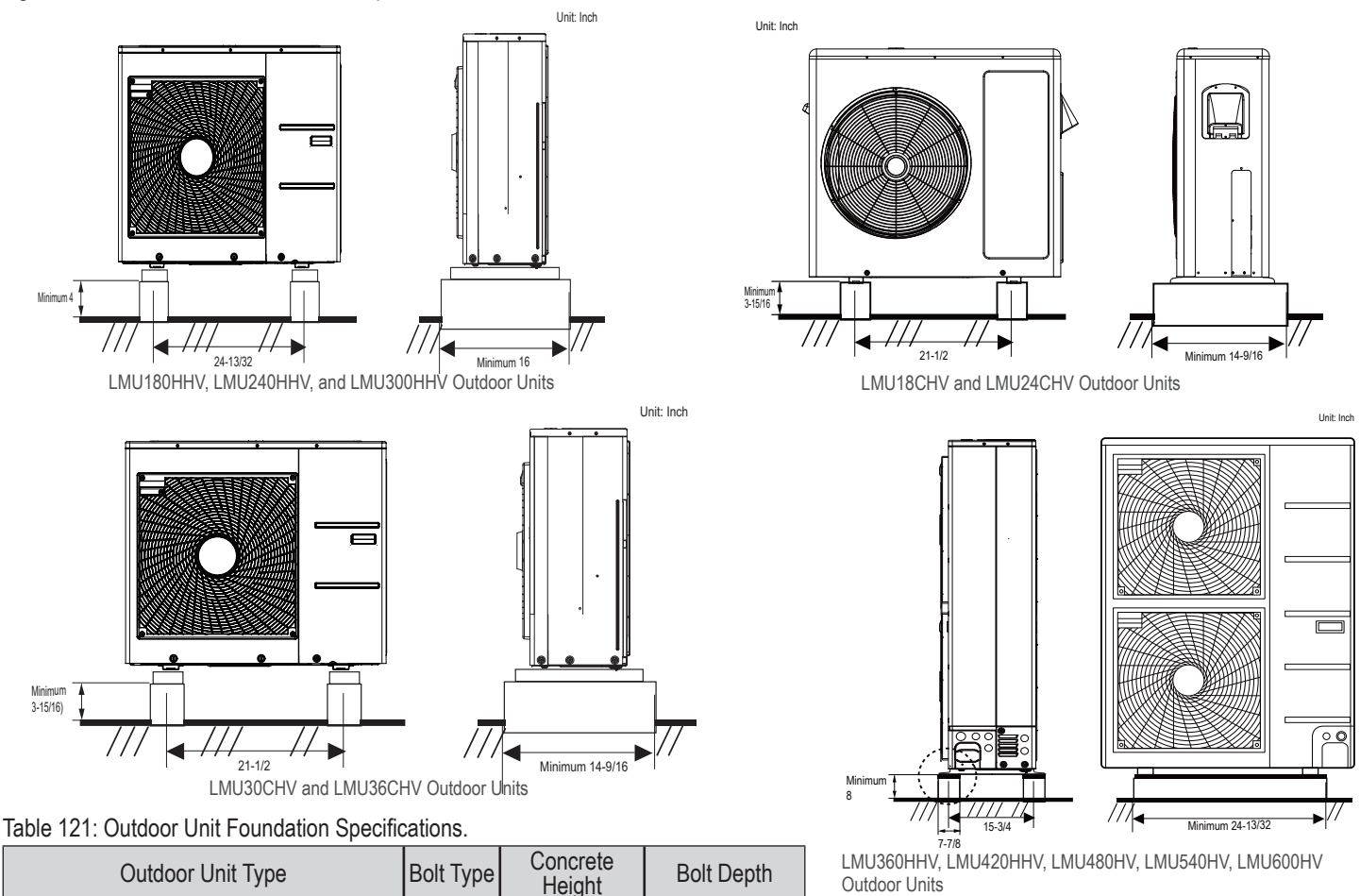
Figure 253: Outdoor Unit Foundation Requirements.
