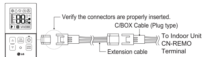
Figure 208:Wired Controller Connections on the Indoor Unit Terminal Block.
