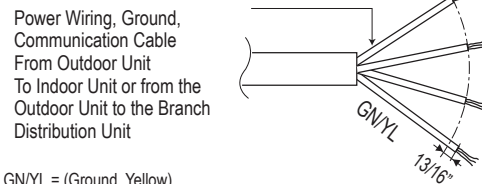
Figure 255: Typical Multi F / Multi F MAX with LGRED Outdoor and Indoor / Branch Distribution Unit Wiring and Communications Cable Diagram For Wiring Lengths Up to 130 Feet.
