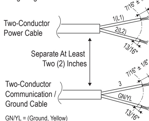
Figure 256: Multi F with LGRED Outdoor Unit to Indoor Unit, and Multi F MAX with LGRED Branch Distribution Unit to Indoor Unit Wiring Diagram for Wiring Lengths GREATER THAN 130 Feet.
