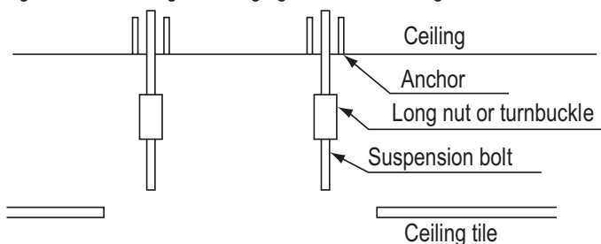
Figure 197: Installing the Hanging Bolt in the Ceiling.
