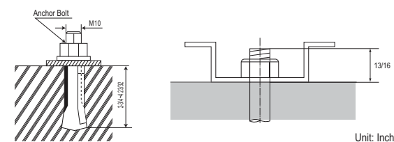
Figure 250: Close up of Bolt Attachment.
