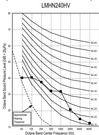
Figure 130: Sound Pressure Level Diagrams.
