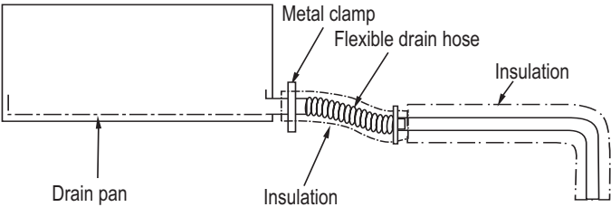
Figure 82: Diagram of an Indoor Unit with a Gravity Drain.
