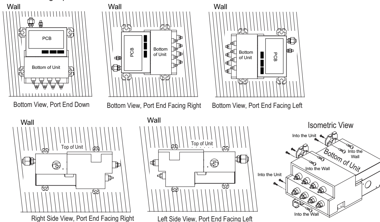
Figure 37: Unacceptable BD Unit Orientation.
