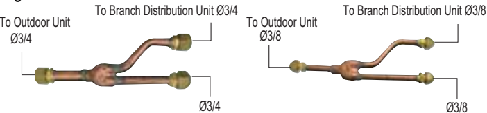
Figure 48: Y-Branch Connections.
