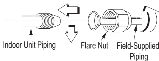
Figure 81: Using the Torque Wrench.
