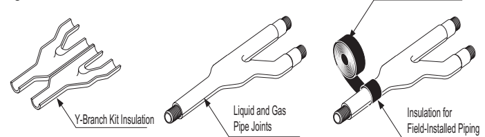
Figure 52: Y-branch Insulation Detail.
