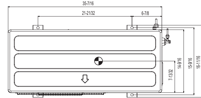
Figure 8: LMU369HV External Dimensions.
