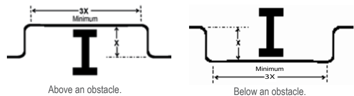
Figure 56: Installing Piping Above and Below an Obstacle.
