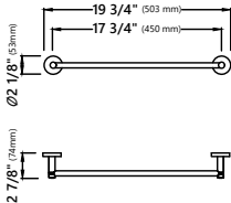
Model #: KEA-18836 Towel Bar Dimensions: 19 3/4" x 2 7/8" x Ø 2 1/8"
