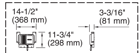
Control Amplifier
