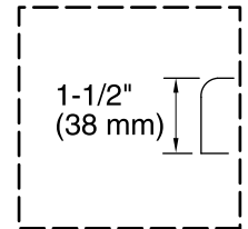
Drop-In Rim Detail
