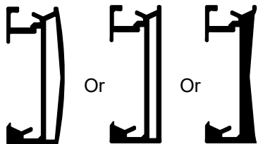
Header (Qty 1)
