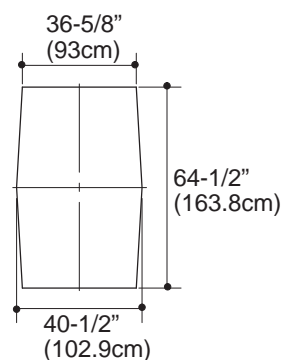
CUT-OUT DETAIL
