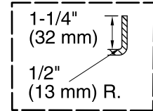
Integral Flange Detail
