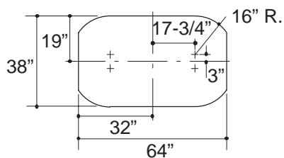
CUT-OUT DETAIL
