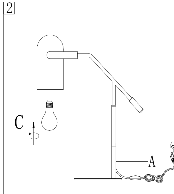
Step 2 Insert the bulb(C) into the socket
