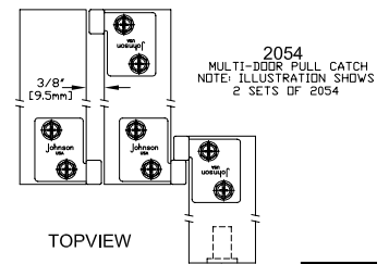
TOPVIEW USE 150 EDGE PULL ON LEAD DOOR
