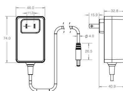
03. POWER ADAPTOR - FRONT & SIDE VIEW
