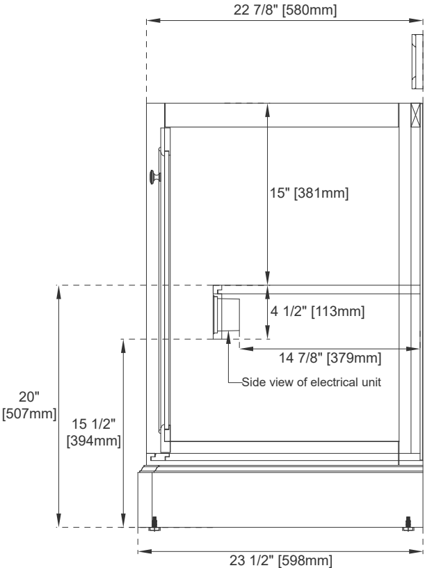
Side View 2
