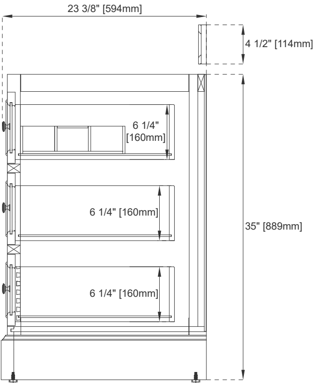
Side View 1
