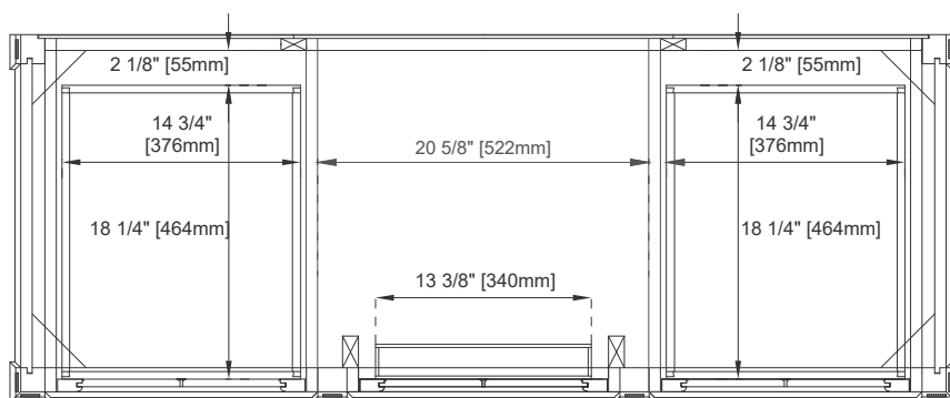
Top View 1
